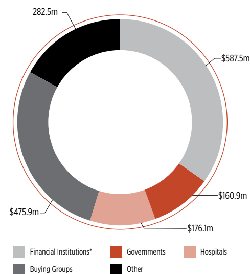
Credit Quality of Financial Assets (30 June 2016)
